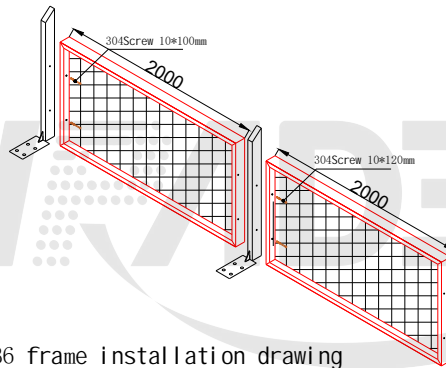
B6 frame installation drawing
