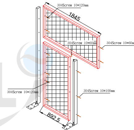
B8/B10 frame installation drawing
