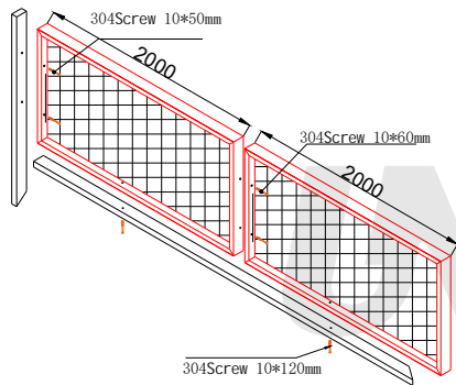
C3 frame installation drawing
